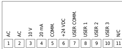
Connections PAXP
